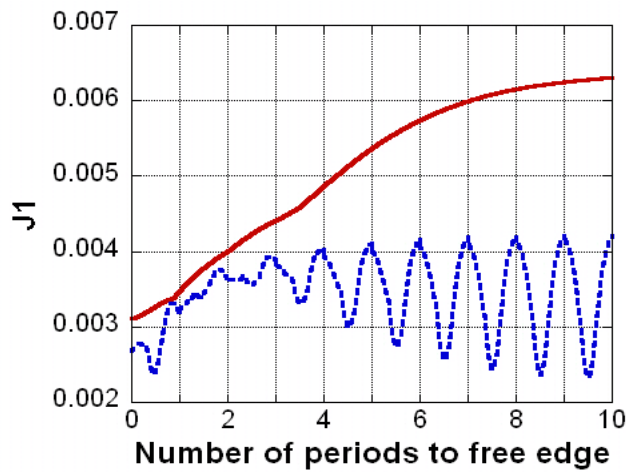
FIG. 7. Comparison of J_1 and (EJ_1)_1 in 0 degree ply 3.0 fiber diameters above the interface.
