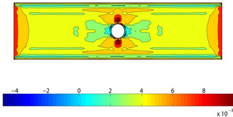
FIG. 16. Bound on the local strain in the 0 degree ply without prestress.
