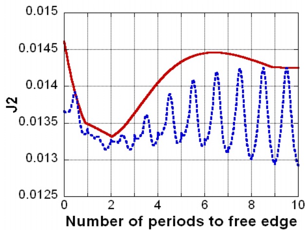
FIG. 8. Comparison of J_2 and (EJ_2)_1 in 0 degree ply 3.0 fiber diameters above the interface.
