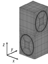
FIG. 4. The choice of S used for computation of the high fidelity asymptotic expansion.
