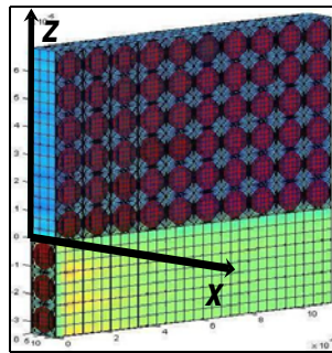
FIG. 3. One slice of a quarter section of a three ply laminate. The slice is one period thick along the x axis.
