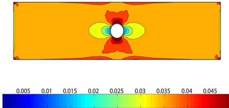
FIG. 21. Bound on the local strain in the 90 degree ply with prestress.
