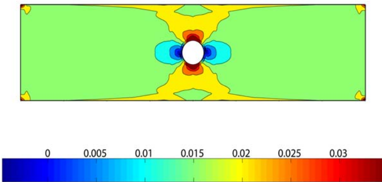
FIG. 20. Bound on the local strain in the 90 degree ply without prestress.
