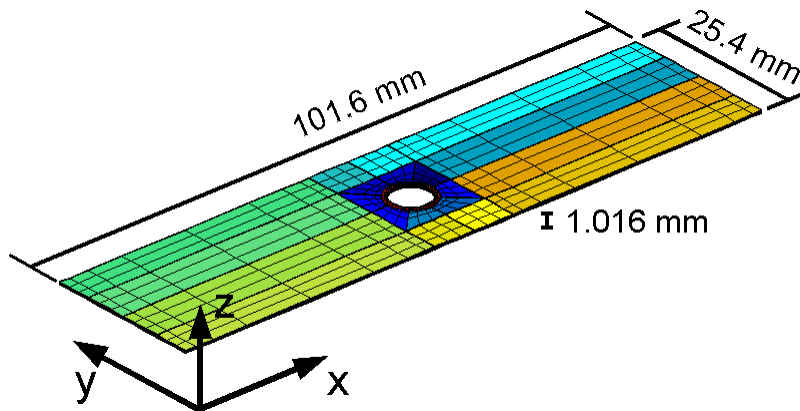
FIG. 15. An open hole eight ply laminate.
