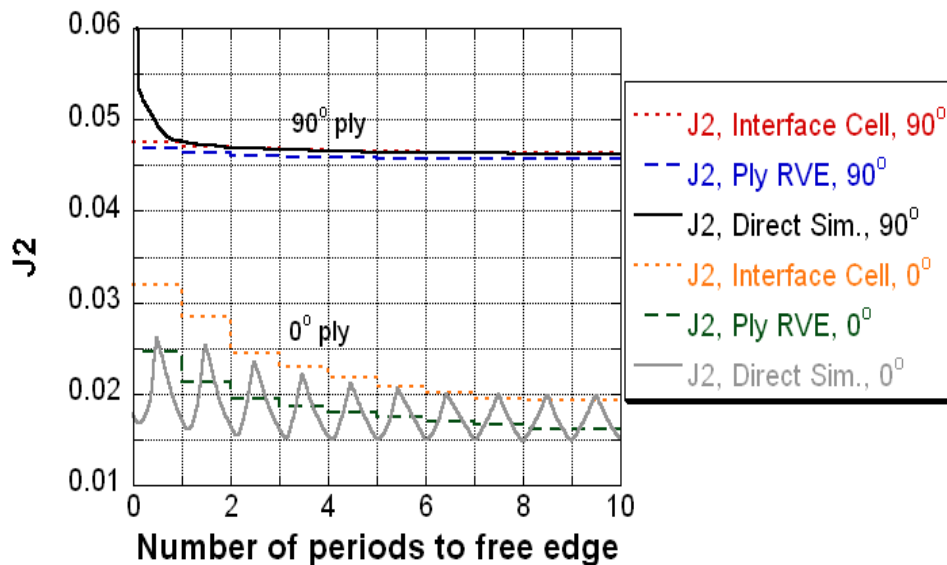
FIG. 5. Comparison between direct numerical simulation and high fidelity asymptotics.
