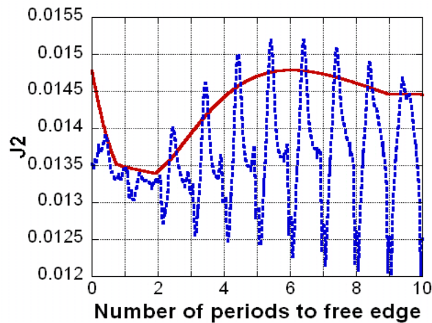
FIG. 10. Comparison of J_2 and (EJ_2)_1 in 0 degree ply 2.5 fiber diameters above the interface.
