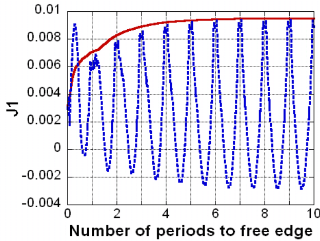
FIG. 13. Comparison of J_1 and (EJ_1)_1 in 0 degree ply 0.5 fiber diameters above the interface.
