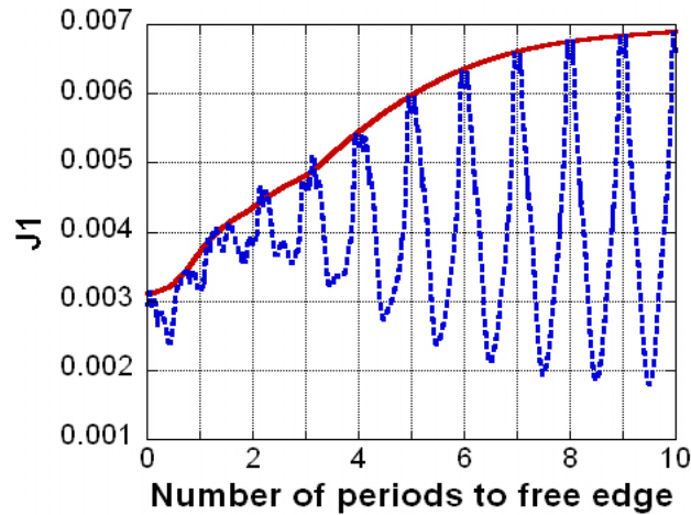
FIG. 9. Comparison of J_1 and (EJ_1)_1 in 0 degree ply 2.5 fiber diameters above the interface.
