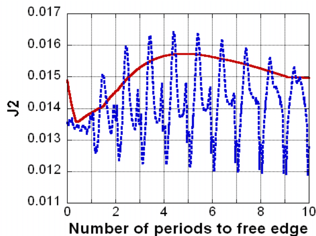
FIG. 12. Comparison of J_2 and (EJ_2)_1 in 0 degree ply 1.5 fiber diameters above the interface.
