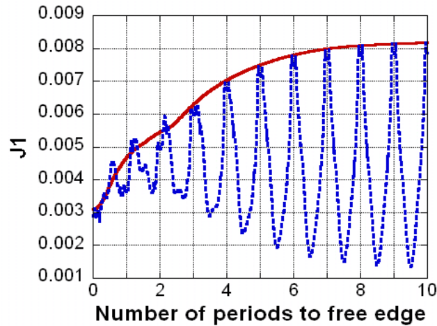
FIG. 11. Comparison of J_1 and (EJ_1)_1 in 0 degree ply 1.5 fiber diameters above the interface.
