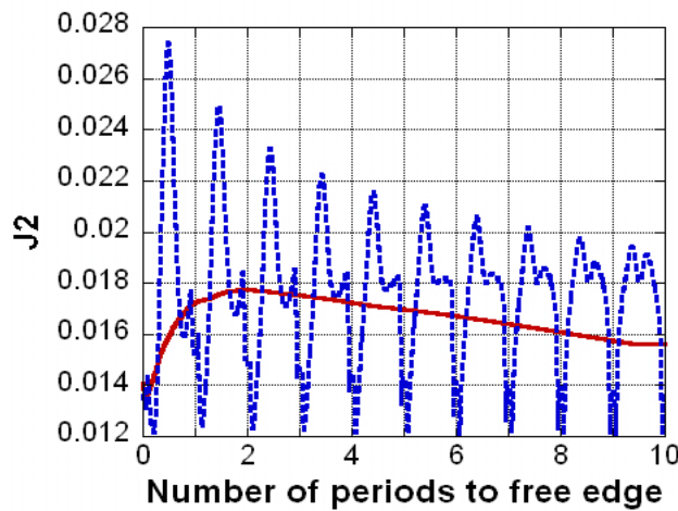
FIG. 14. Comparison of J_2 and (EJ_2)_1 in 0 degree ply 0.5 fiber diameters above the interface.
