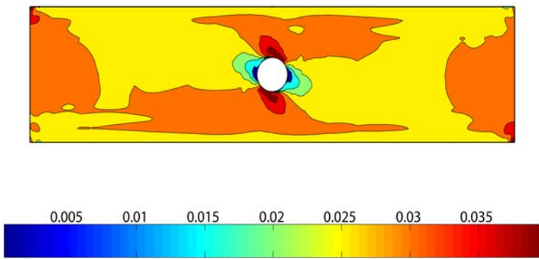
FIG. 19. Bound on the local strain in the 45 degree ply with prestress.
