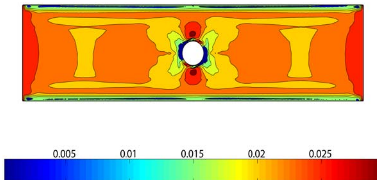
FIG. 17. Bound on the local strain in the 0 degree ply with prestress.
