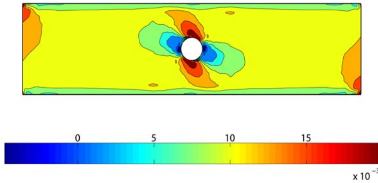
FIG. 18. Bound on the local strain in the 45 degree ply without prestress.
